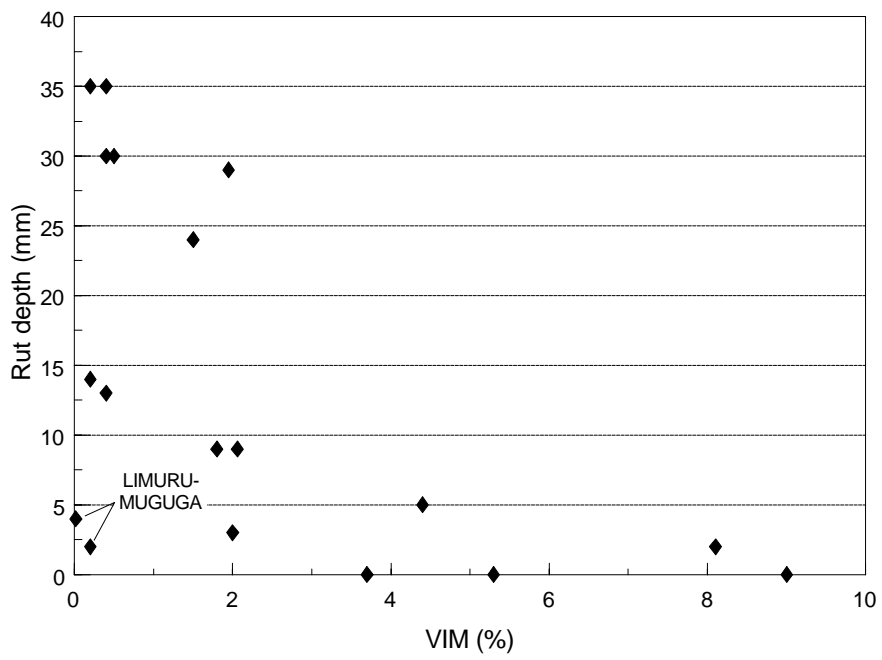
Figure 2 Relationship between VIM and rut depth
